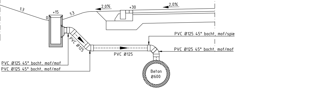
Principedetail slok-op
